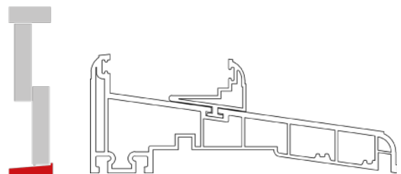
Flush Cill
