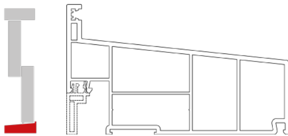
Deep Flush Cill
