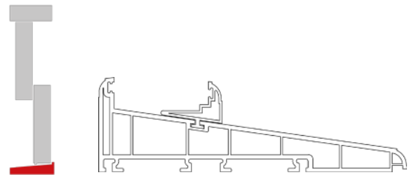
180mm Protruding Cill
