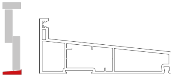
Flush Cill
