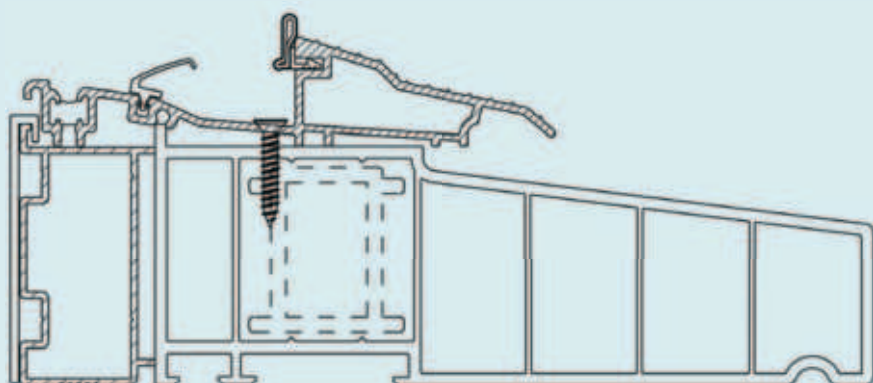
55MM RADLINGTON CILL
