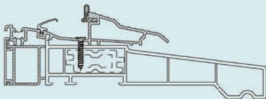
30MM RADLINGTON CILL
